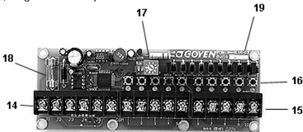
Figure 4: PS-L, Large Terminal Expansion Card
