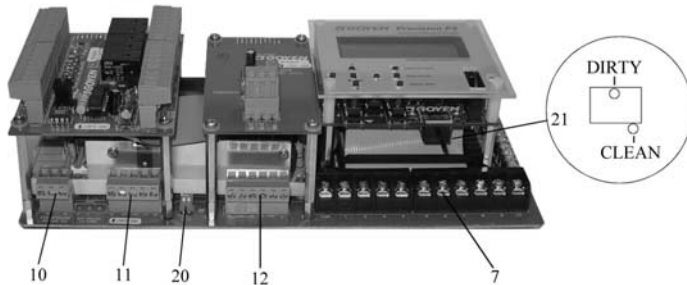
Figure 2: Controller Assembly, Front View
