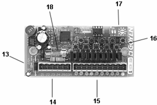
Figure 4: PS-L, Large Terminal Expansion Card
