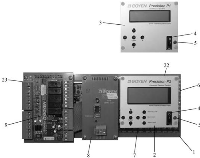
Figure 2: Controller Assembly, Front View
